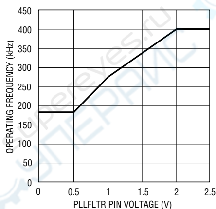
Figure 7. Frequency vs PLLFLTR Pin Voltage
